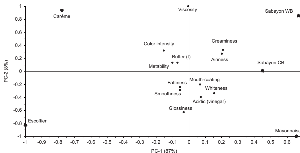
Fig. 5. Principal component analysis (PCA) bi-plot of sensory results. 95% of the variance was explained by the first two components. Only significant descriptors are plotted. “Historic” (Car me and Escoffier) sauces to the left and «modern» sauces (Sabayon WB, Sabayon CB and Mayonnaise) to the right. Stars and dots represent sauces and descriptors respectively.
